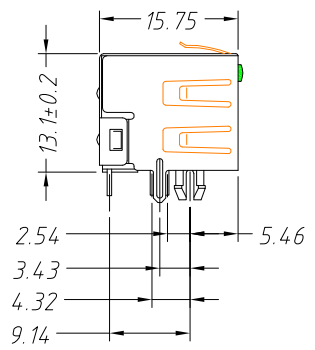
With EMI Shield
